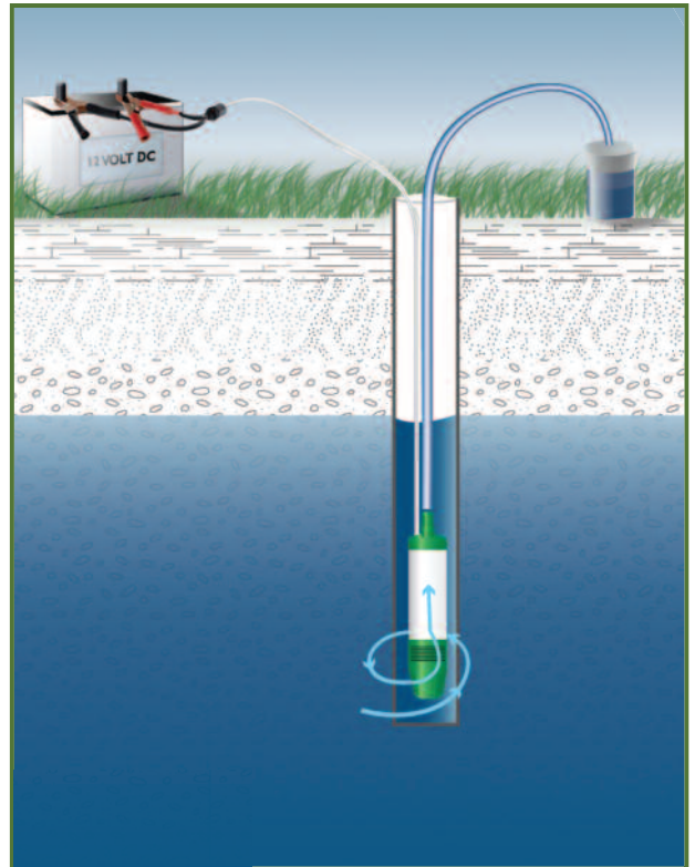
STANDARD PERFORMANCE PUMP IN ACTION
